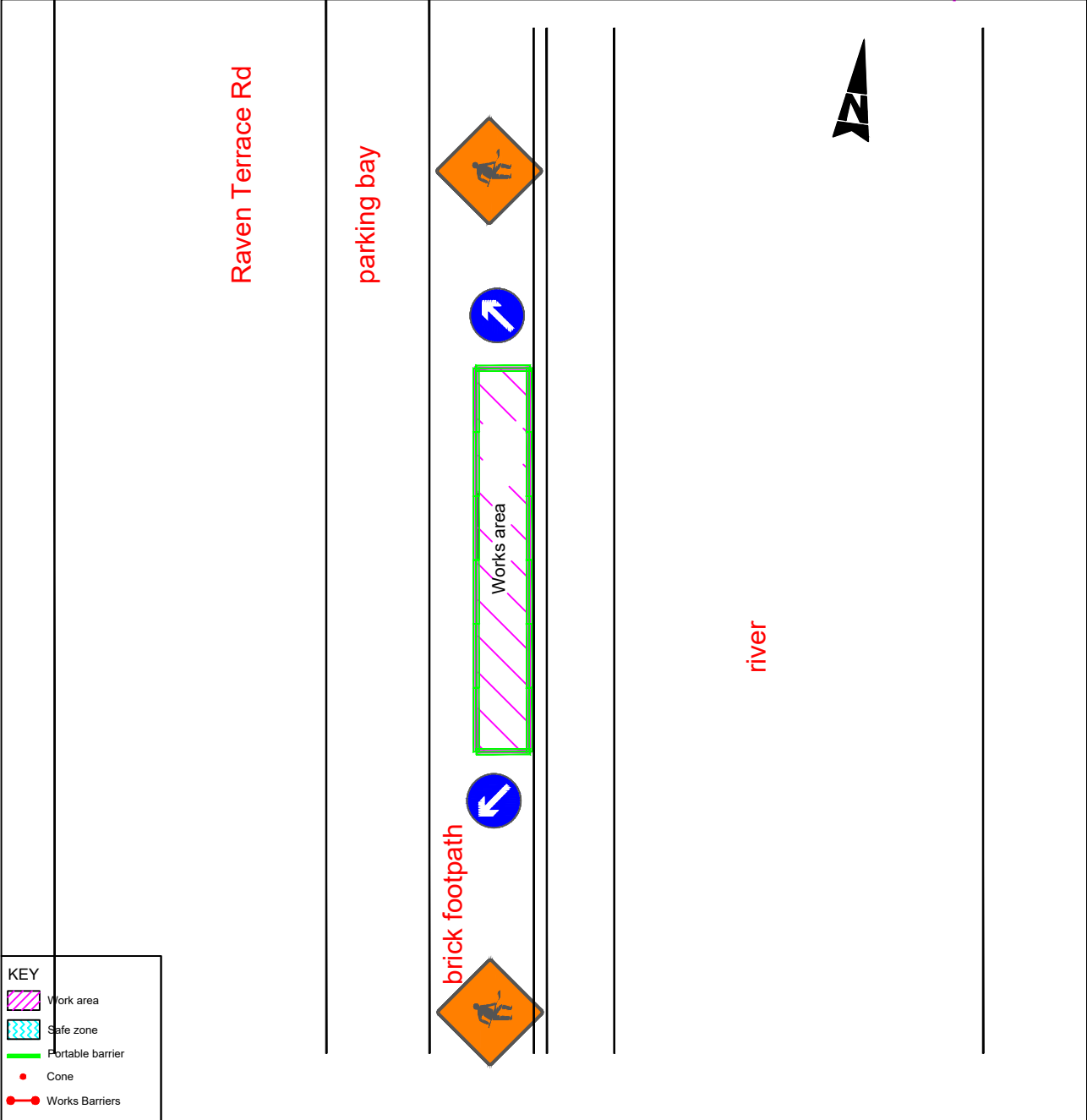
LOCATION PLAN, 1:100 ON A4
